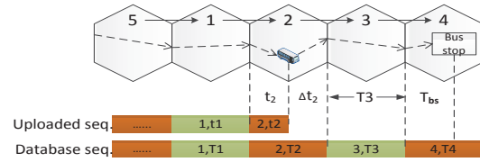
Fig. 13. Bus arrival time prediction
