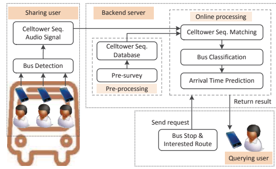
Fig. 2. System architecture
