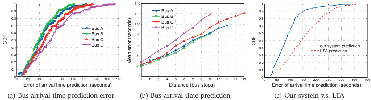
Fig. 17. Arrival time prediction performance
