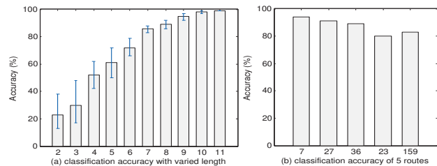
Fig. 19. Bus classification results
