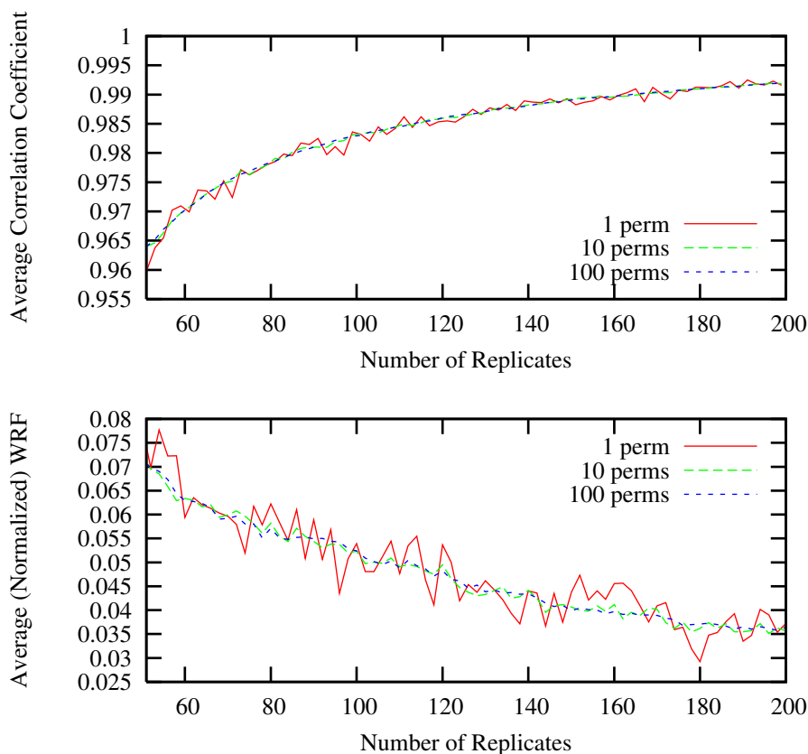
Fig. 1. FC (top) and WC (bottom) criteria for various p settings on dataset 500
