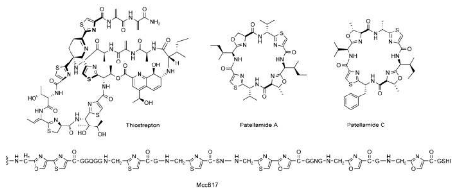
Figure 7. Examples of antibiotic peptides that contain five-membered heterocycles derived from cysteine or serine/threonine. The first twelve residues of MccB17 (VGIGGGGGGGG) are omitted.
