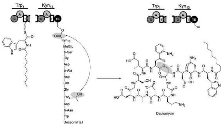
Figure 23. Truncated depiction of the daptomycin assembly line illustrating modules 1 and 13. Macrocyclization of the 13-mer peptide by the TE domain results in chain release and daptomycin formation.
