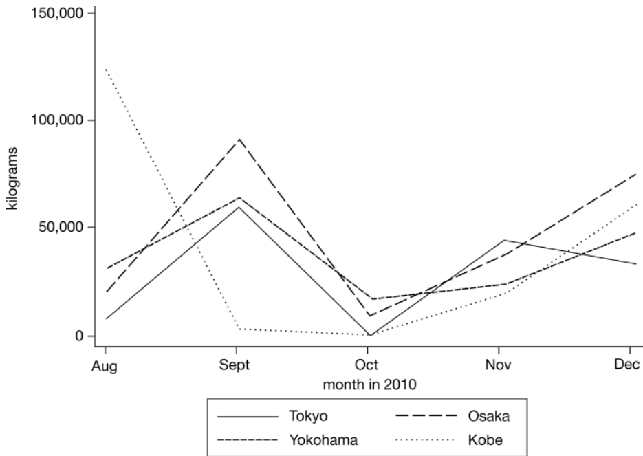
Figure 10. Miscellaneous Rare Earth Metals
