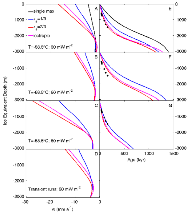
Figure 4. (A–D) Vertical velocity, w , as a function of depth from the surface to bedrock for different fabrics, surface temperature and geothermal heat flux at Kunlun station. (A–C) are steady-state simulations using fabric as in the key of (A). Surface temperatures and geothermal heat fluxes and surface temperatures are labelled on the panels. (D) is for the transient simulations with time-varying surface temperature (Table 1) from 130 kyr BP. (E–G) Age–depth profile at Kunlun station corresponding to the simulations in the left column. The black points denote the age–depth data from dated radar internal reflection horizons tracked from the Vostok ice core site, using a 46 m firn correction subtracted from the radar depths to convert to the ice-equivalent model scale. No age calculation is possible for the short transient runs, but the expected ages may be judged by relation to the steady-state w simulations.
