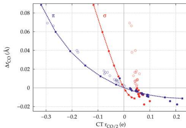
Fig. 8 The dashed lines show \Delta r_{\text{CO}} versus the \sigma (red color) and \pi (blue) CO polarization \text{CT}_{r_{\text{CO}/2}} for a CO molecule placed in a uniform axial electric field of magnitude ranging from -0.11 to 0.07 a.u. in steps of 0.02 a.u. (colored square points). For comparison, also shown is the correlation between \Delta r_{\text{CO}} and \sigma and \pi CO polarization (red and blue circles, respectively) for the whole series of Au and homoleptic complexes studied. The empty circles are for neutral or negatively charged complexes, the filled circles for cationic ones.
