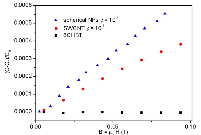
Fig. 3. Relative capacitance variation vs. magnetic field for undoped 6CHBT and 6CHBT doped with spherical \text{Fe}_3\text{O}_4 nanoparticles or with SWCNT.
