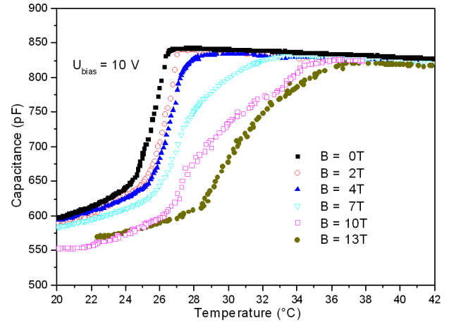
Fig. 7. Temperature dependence of the capacitance of the sample (molar fraction of 6CHBT is 0.906) doped with magnetic particles at volume concentration of \Phi = 5 \times 10^{-4} , for U_{\text{bias}} = 10 V < U_c and external magnetic fields B = 0, 2, 4, 7, 10 and 13 T. (The magnetic field is applied perpendicular to the electric field).
