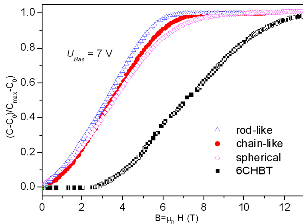
Fig. 2. Dependence of the reduced capacitance of undoped 6CHBT and 6CHBT doped with spherical, chain-like and rod-like particles on the external magnetic field measured at a bias voltage of U_{\text{bias}} = 7 V.
