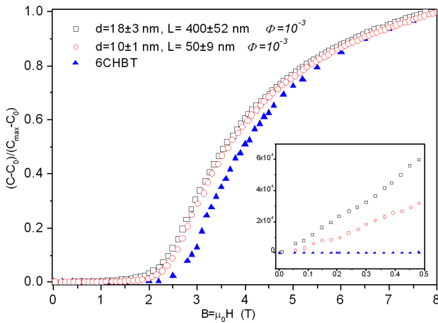
Fig. 4. Reduced capacitance versus magnetic field for undoped 6CHBT and 6CHBT doped with rod-like particles of different size. The inset represents the blowup of the low magnetic field range.
