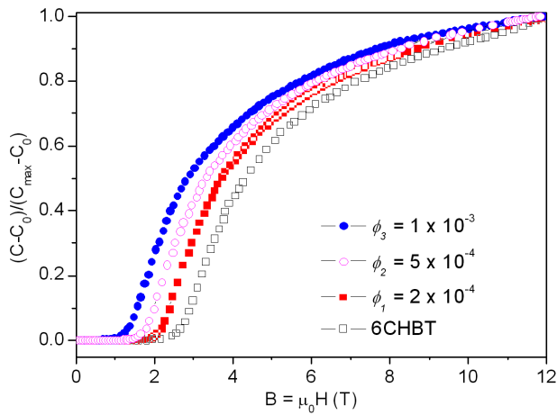
Fig. 1. Reduced capacitance versus magnetic induction for undoped 6CHBT and for 6CHBT doped with different volume concentrations of spherical magnetic nanoparticles.
