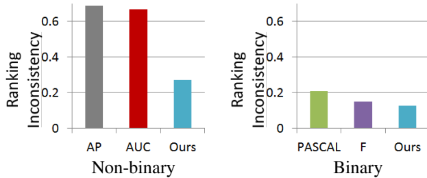
Figure 9. Meta-measure 1 – results: The ranking correlation of an evaluation measure to that given by the image retrieval application. The results presented are 1 - \rho ( \rho denoting Spearman’s Rho measure). The lower the score, the better an evaluation measure is at predicting the preference of the application. Our measure offers improvement over the other measures.
