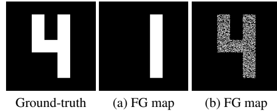
Figure 4. Dependency flaw. (a-b) are two binary maps with the same TP, TN, FP and FN values. Current measures consider each pixel as independent. Hence, they ignore the fact that the false-negatives in (b) are sparsely spread within true-positive detections, thus offering a good sampling of the foreground region.
