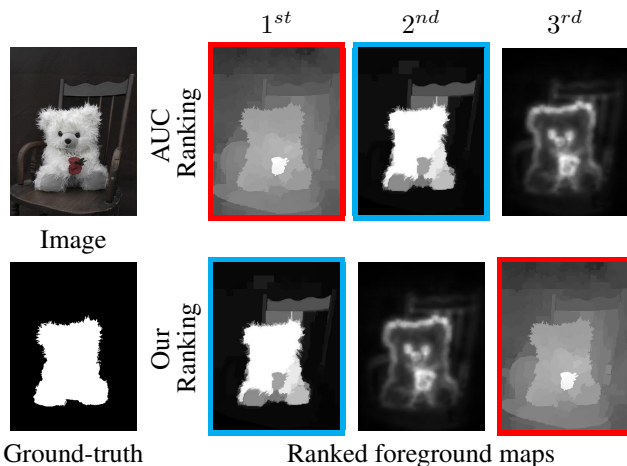
Figure 1. Inaccuracy of current evaluation measures. We compare the ranking of foreground maps that are the output of three state-of-the-art salient-object detection algorithms [9, 12, 13]. According to the most common measure, AUC, the red map offers the best result despite its fuzziness, which captures much of the background. Conversely, our proposed measure correctly ranks first the cyan map, which most accurately captures the foreground object, according to the ground-truth. Our ranking is supported by four meta-measures.
