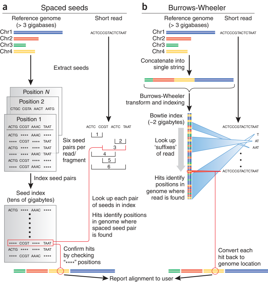
Figure 1 Two recent algorithmic approaches for aligning short (20–200-bp) sequencing reads. (a) Algorithms based on spaced-seed indexing, such as Maq, index the reads as follows: each position in the reference is cut into equal-sized pieces, called ‘seeds’ and these seeds are paired and stored in a lookup table. Each read is also cut up according to this scheme, and pairs of seeds are used as keys to look up matching positions in the reference. Because seed indices can be very large, some algorithms (including Maq) index the reads in batches and treat substrings of the reference as queries. (b) Algorithms based on the Burrows-Wheeler transform, such as Bowtie, store a memory-efficient representation of the reference genome. Reads are aligned character by character from right to left against the transformed string. With each new character, the algorithm updates an interval (indicated by blue ‘beams’) in the transformed string. When all characters in the read have been processed, alignments are represented by any positions within the interval. Burrows-Wheeler-based algorithms can run substantially faster than spaced seed approaches, primarily owing to the memory efficiency of the Burrows-Wheeler search. Chr., chromosome.
