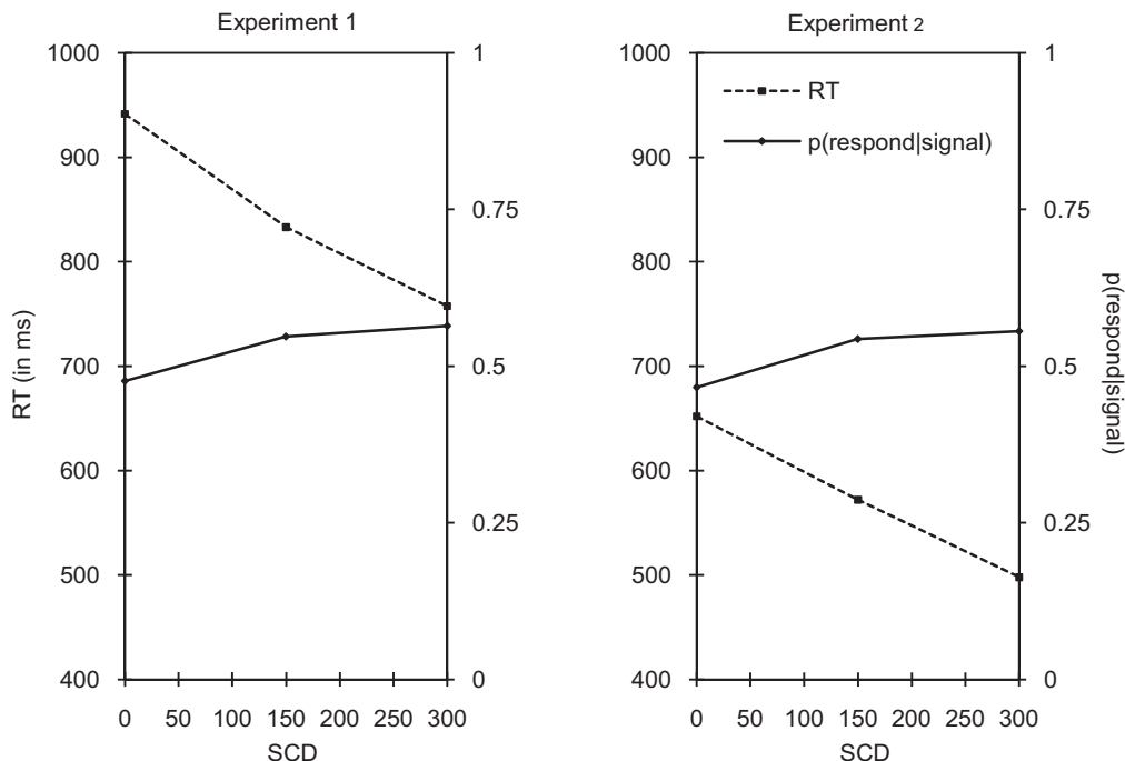
Figure 5. Mean GO2 reaction times (RTs; left y-axis) and probabilities of responding ( p(\text{respond}|\text{signal}) ; right y-axis) as a function of SCD (in ms) in Experiment 1 (left panel) and Experiment 2 (right panel). The dotted lines represent the GO2 RTs, and the solid lines represent the p(\text{respond}|\text{signal}) .
