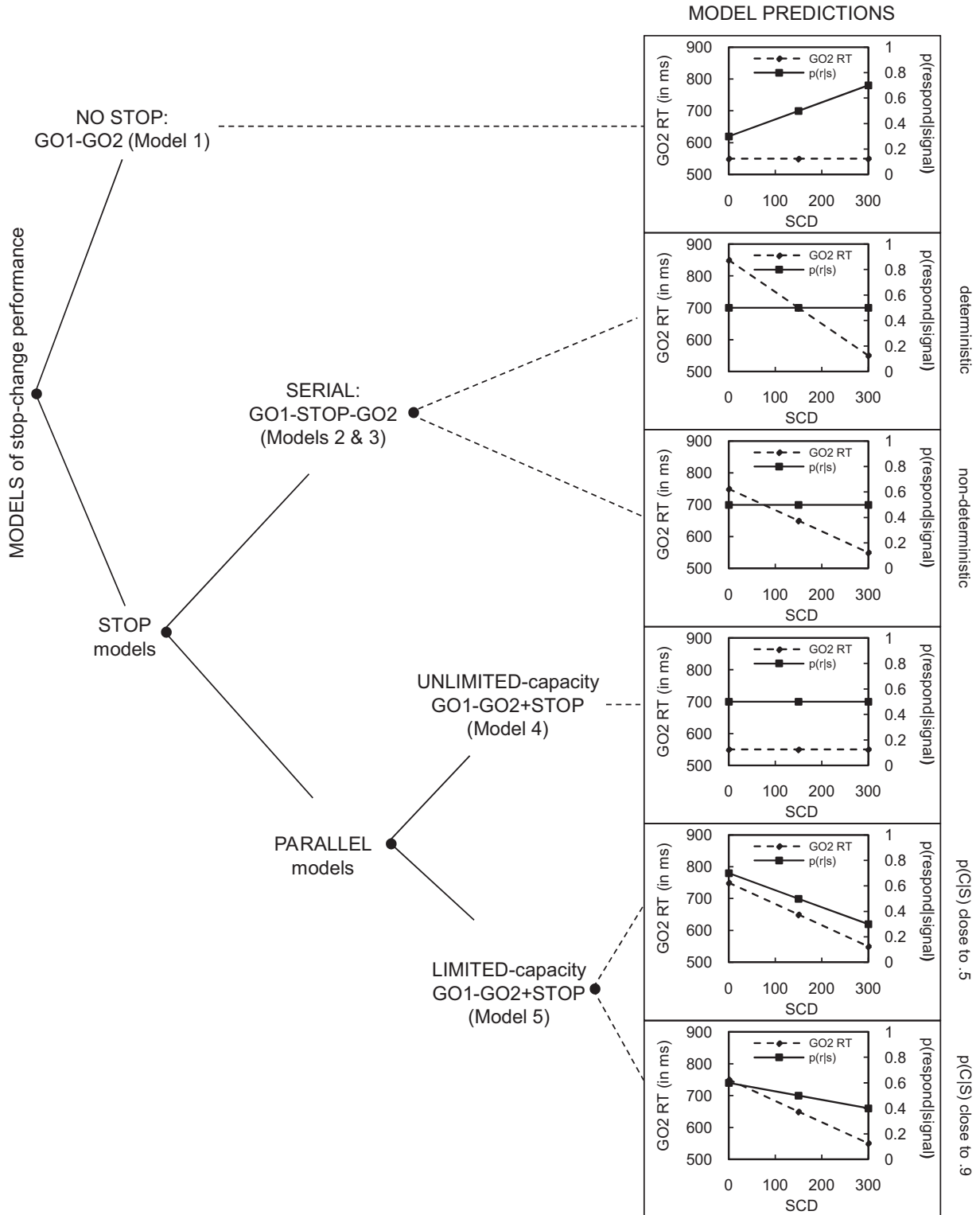
Figure 2. The different models and their predictions for probability of responding, p(r/s) , and GO2 reaction time (RT) as a function of stop-change delay (SCD: 0, 150, or 300 ms). For the limited-capacity model, p(c|s) is the proportion of capacity allocated to the STOP process. See text for further details.
