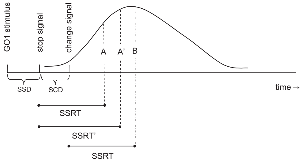
Figure 3. Illustration of the predicted probabilities of responding, p(\text{respond}|\text{signal}) , based on the horse-race model (Logan & Cowan, 1984), given the distribution of GO1 reaction times (GO1 RT) and the stop-signal reaction time (SSRT). The p(\text{respond}|\text{signal}) is represented by the area under the curve to the left of each dashed line, which increases if SSRT is prolonged (compare Lines A and A') or if subjects do not stop until the change signal is presented (compare Lines A and B).
