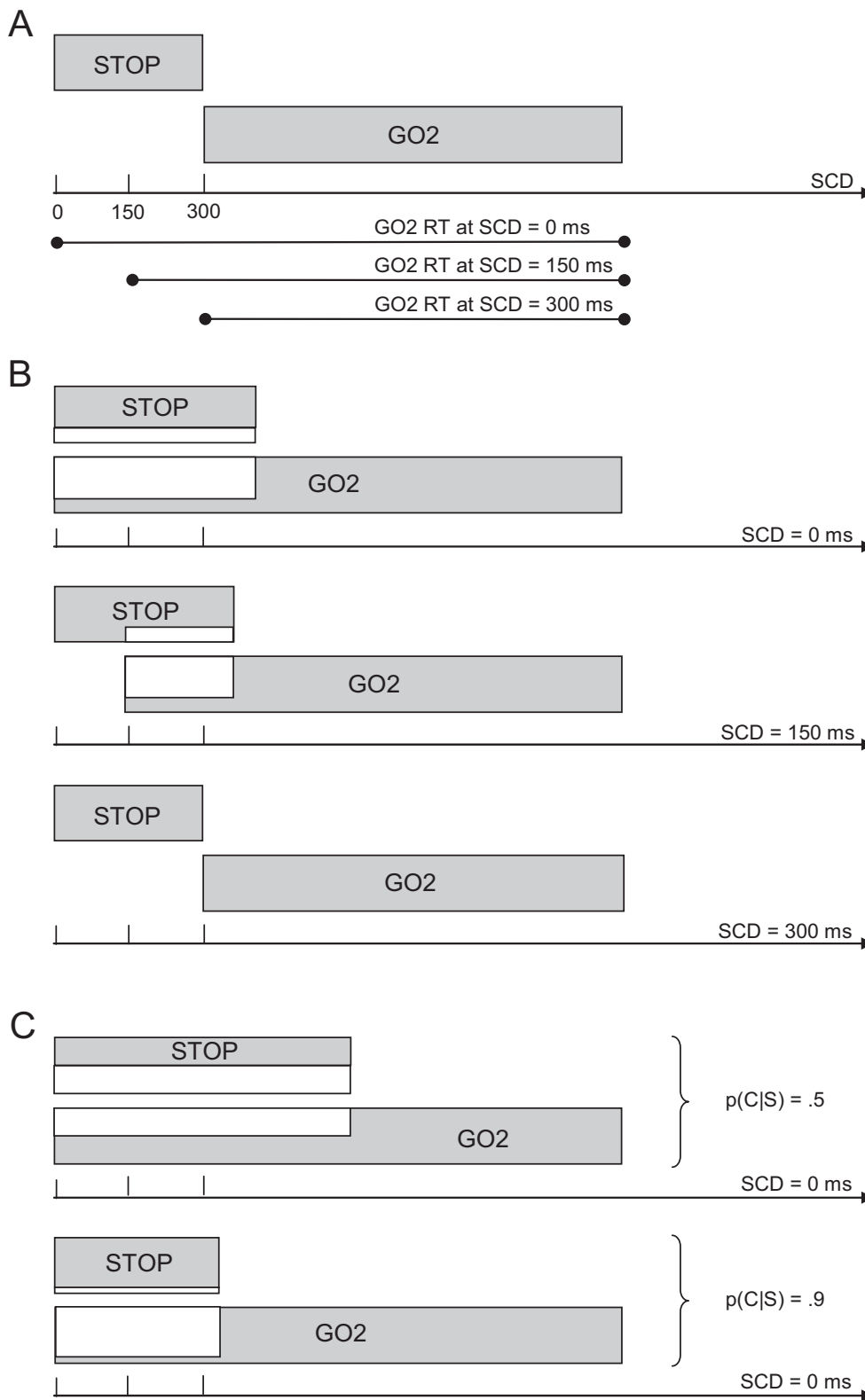
Figure 4. Stage diagrams for the STOP and GO2 processes as a function of stop-change delay (SCD) for the GO-STOP-GO models (A) and the limited-capacity GO-GO+STOP model (B). The length of each box represents the duration of each stage. White areas represent shared capacity. See text for further details. Stage diagrams for the STOP and GO2 processes as a function of the proportion of capacity allocated to the STOP process, p(c|s) , for SCD = 0 ms (C).
