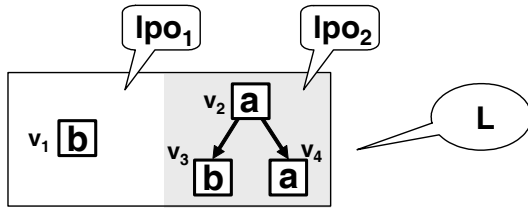
Figure 6: A partial language L = \{lpo_1, lpo_2\} with W = \{v_1, v_2, v_3, v_4\} and E = \{(v_2, v_4), (v_2, v_3)\} .
