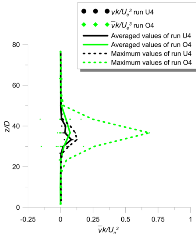
Figure 9. Values of \bar{\nu}k of runs U4 and O4 of the transversal section at x/D=26.67 with the lines of the averaged-values and the maximum-values.
