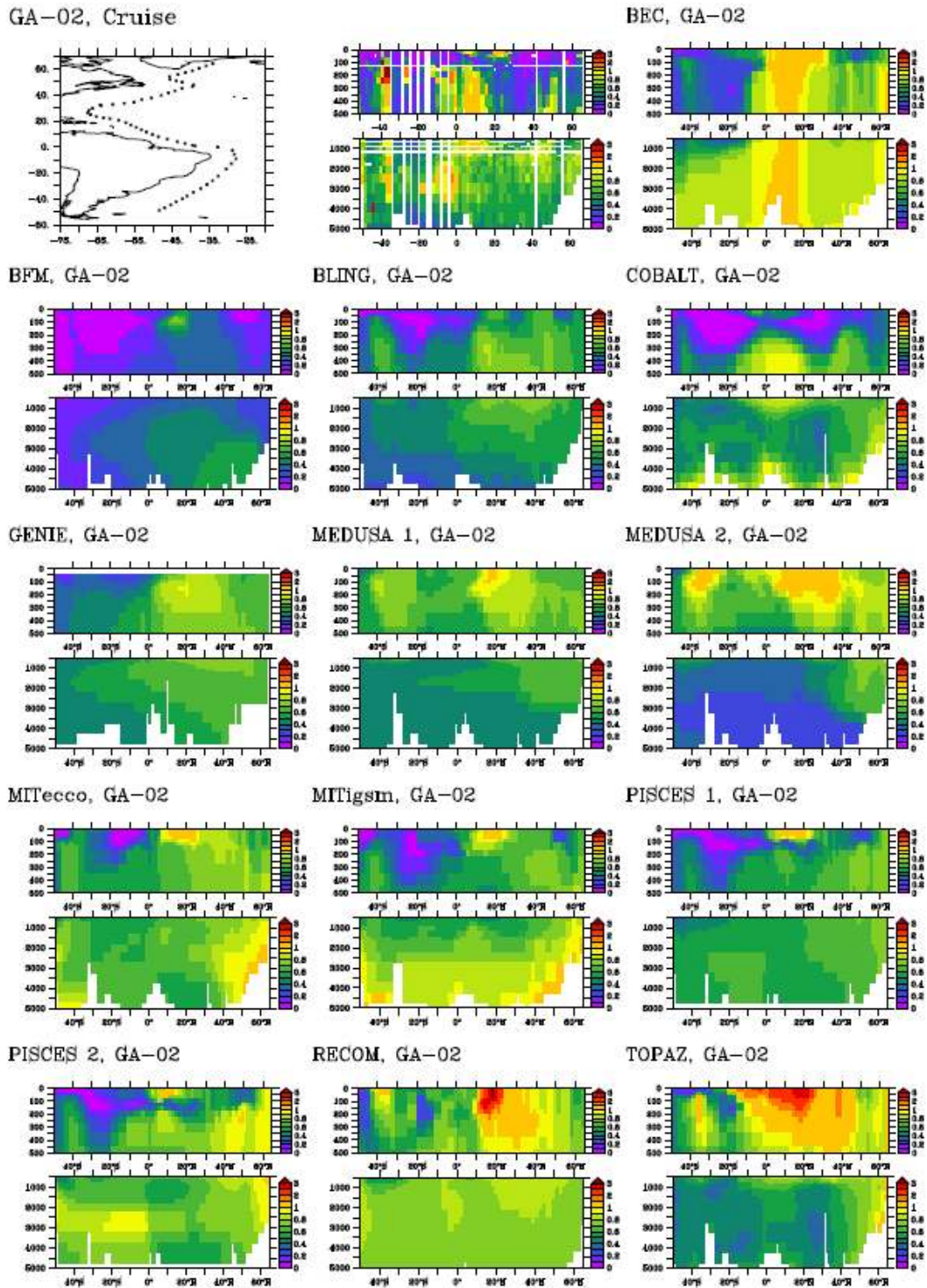
Figure 4. DFe concentrations (nM) from the GA-02 [Rijkenberg et al. , 2014] cruise and extracted from the FeMIP models.
