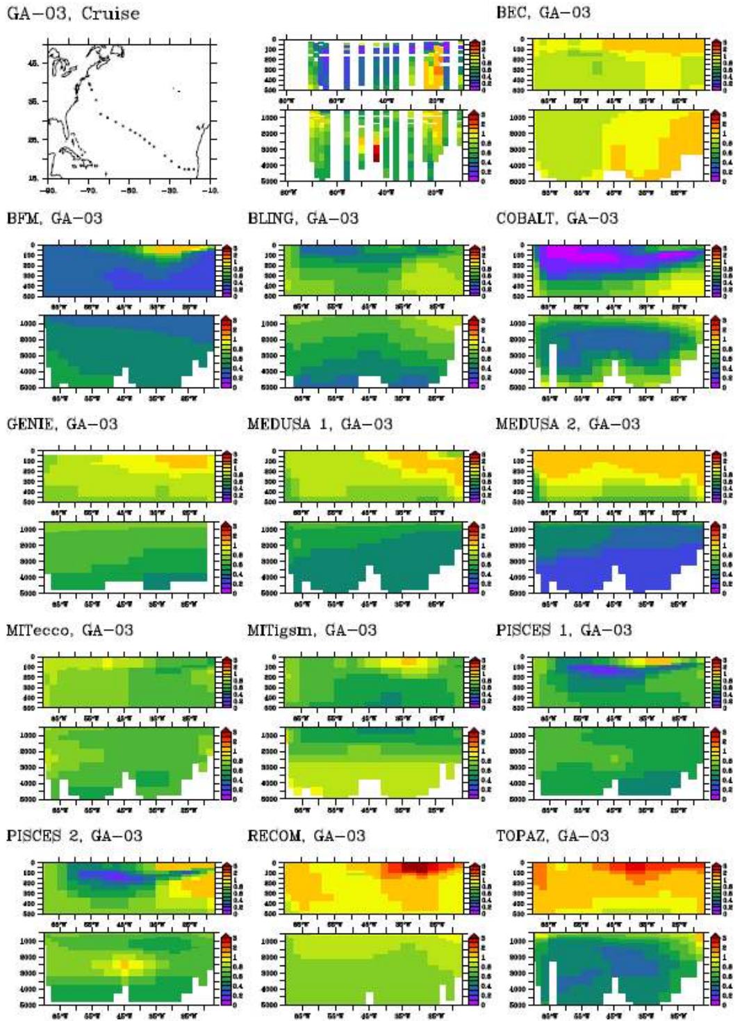
Figure 5. DFe concentrations (nM) from the GA-03 cruise [Hatta et al. , 2014] and extracted from the FeMIP models.
