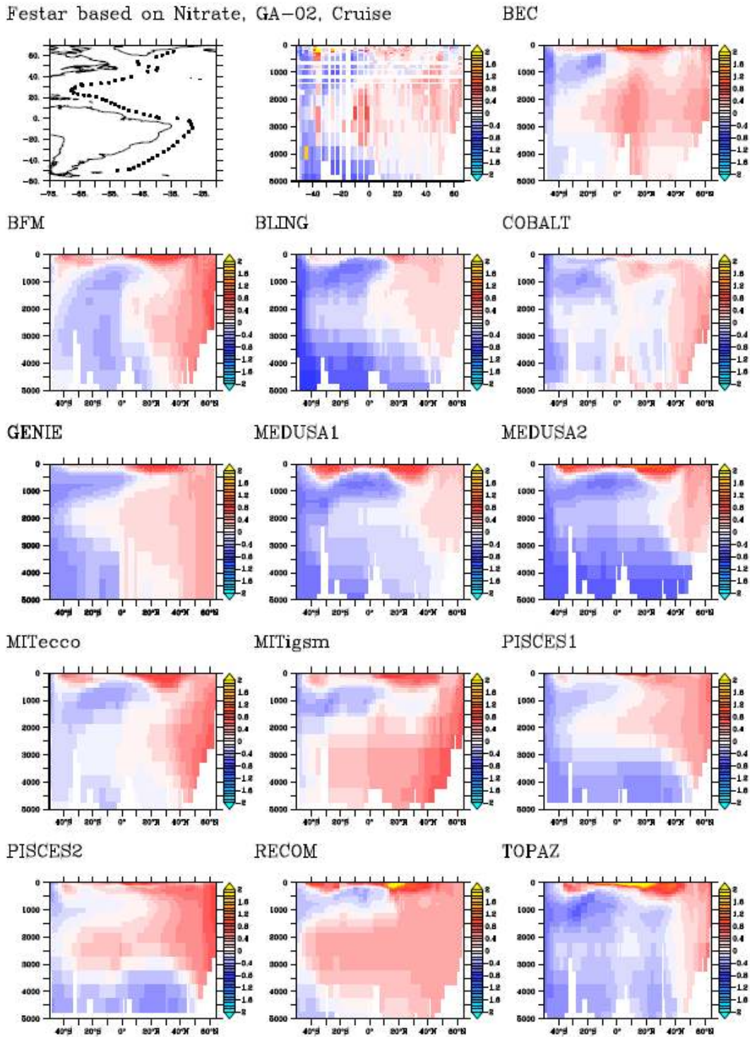
Figure 11. Fe^* ( Fe - NO_3^* r_{Fe/N} , nM) from the GA-02 cruise [Rijkenberg et al. , 2014] and extracted from the FeMIP models. For models that do not provide NO_3 , PO_4 is used and converted to NO_3 assuming a ratio of 16:1.
