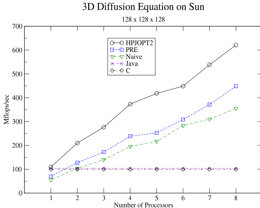
Figure 9. Three dimensional Diffusion equation with size of 128 x 128 x 128 on SMP.
