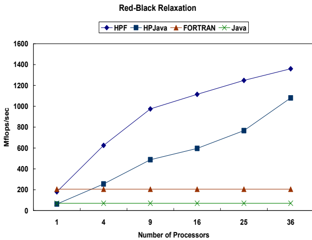
Figure 7. Laplace Equation with red-black relaxation with size of 512 x 512 on IBM SP3.
