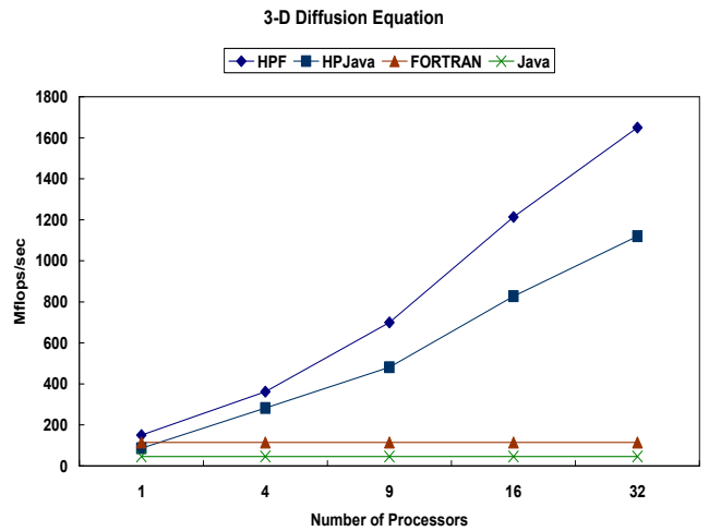
Figure 8. Three dimensional Diffusion equation with size of 128 x 128 x 128 on IBM SP3.
