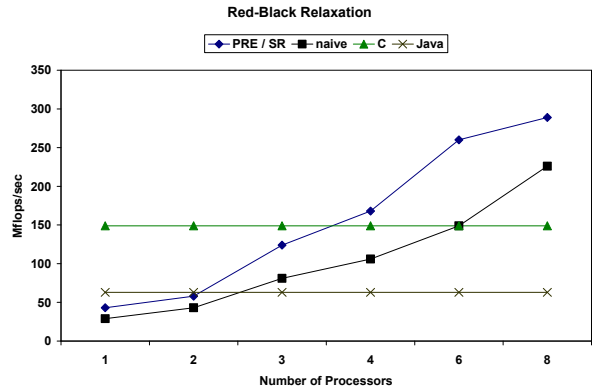
Figure 6. Laplace Equation with red-black relaxation with size of 512 x 512 on Sun Solaris 9 with 8 UltraSPARC III processors.
