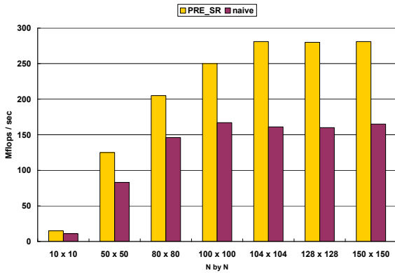
Figure 5. Experiment for matrix multiplication in HPJava with PRE/SR.
