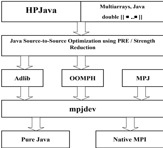
Figure 4. HPJava Architecture.
