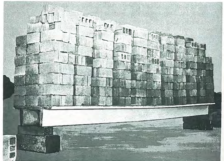
Fig. 11. The first load test on a 14-in. (356 mm) deep, 4-ft (1.2 m) wide and 25-ft (7.6 m) long double-tee. Note the small deflection. Span lengths were later increased to 50 ft (15.3 m).
