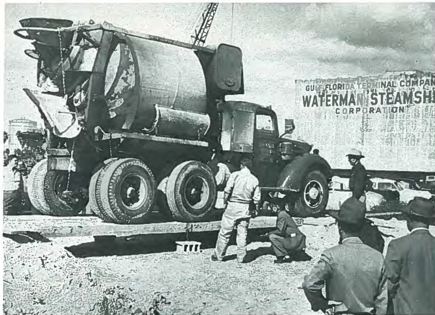
Fig. 24. Demonstration test by Cone Brothers Construction Co. in Tampa, Florida (1954) of 2-in. (51 mm) thick prestressed slab with 4-in. (102 mm) composite topping. The span was 30 ft (9.2 m) long.
