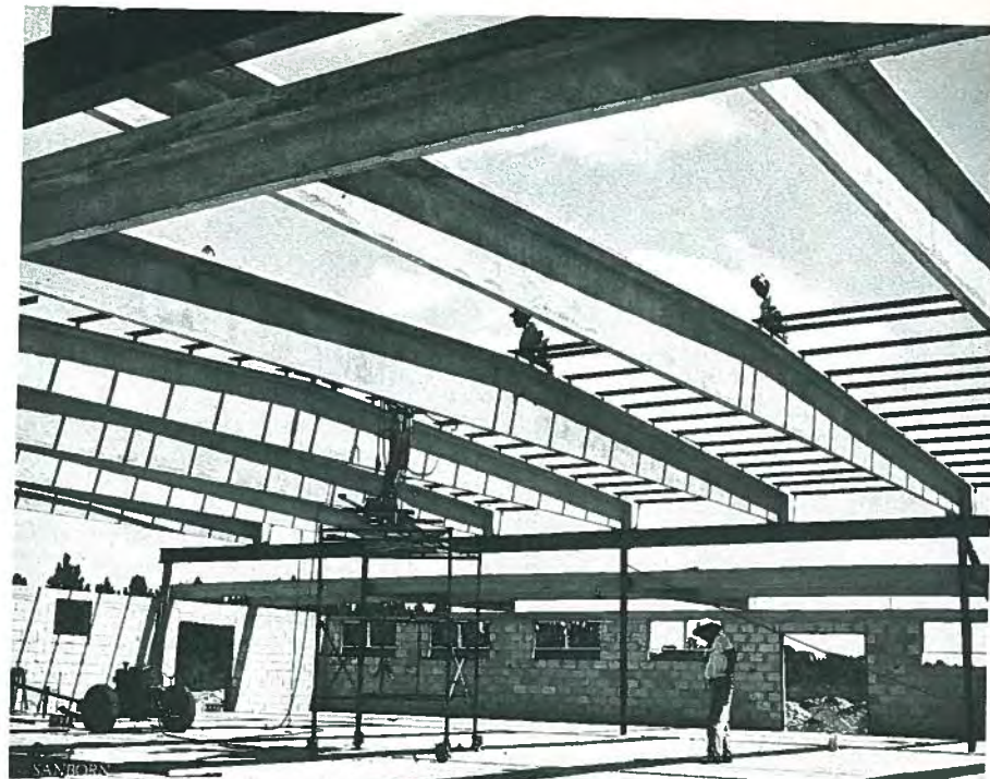
Fig. 4. One of the first examples of pretensioned tapered beams built in Florida in the mid-fifties. These 60-ft (18.3 m) beams were fabricated by Prestressed Concrete Inc., in Lakeland.
