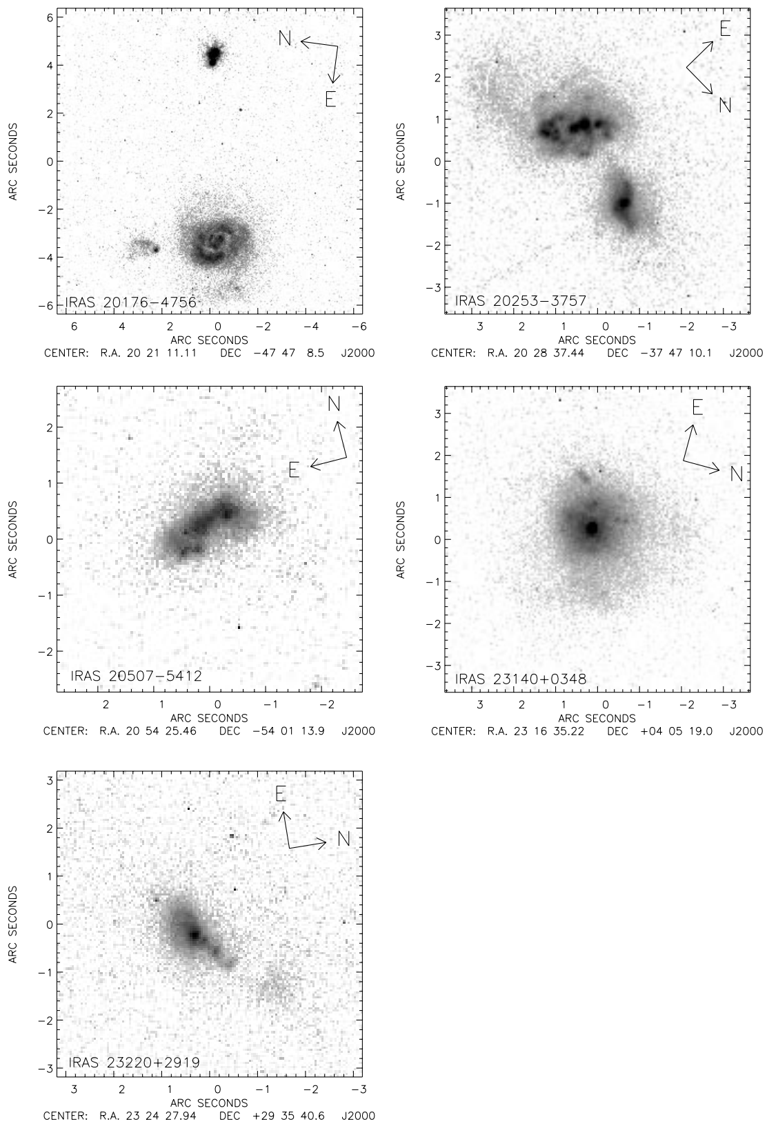
Figure 4. HST F606W images of IRAS 20176-4756 to IRAS 23220+2919.
