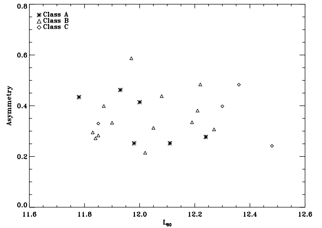
Figure 10. 60- \mu\text{m} luminosity plotted against asymmetry for all 23 ULIRGs. Description of the classes A, B and C can be found in Section 4.1.
