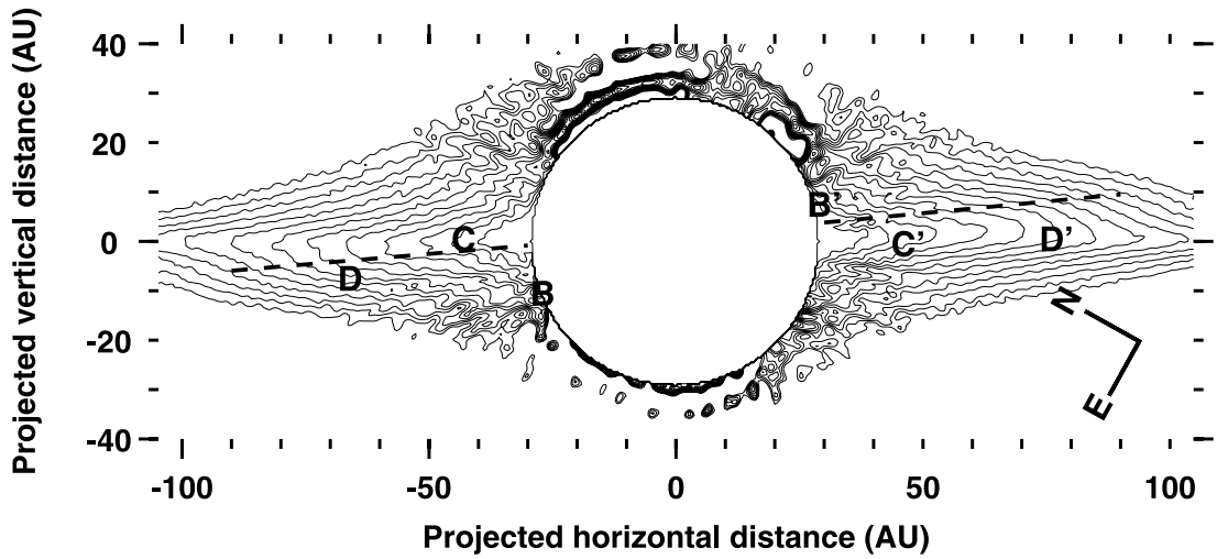
FIG. 12.—Isophotal map of the inner region of the disk obtained from our PSF-deconvolved F606W image. The data have been smoothed with a 3 \times 3 pixel boxcar. The isophotes represent surface brightnesses of 10\text{--}15.4 mag arcsec ^{-2} at intervals of 0.2 mag arcsec ^{-2} . The dashed lines are the best linear fits to the spine of the secondary disk. The locations of the diametrically opposed clumps of 18\ \mu\text{m} emission are marked with the letters assigned to them by Wahhaj et al. (2003). The bright clump of emission reported by Telesco et al. (2005) is nearly coincident with clump C'. No such clumping is evident in scattered optical light.
