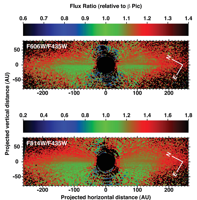
FIG. 17.—F606W/F435W and F814W/F435W ratio images of the composite disk after PSF deconvolution. The images have been smoothed with a 7 \times 7 pixel boxcar. The flux ratios are measured relative to those of the star in the respective bandpasses. Within 150 AU of the star, the uncertainties in the flux ratios range from \sim 5\% to 10\% along the spine of the disk to \sim 25\% at projected distances of \pm 50 AU from the spine. The F814W/F606W image is not shown but is qualitatively similar to the F606W/F435W and F814W/F435W images.
