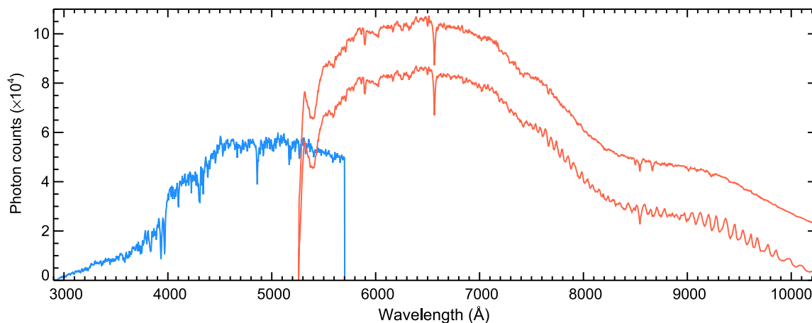
Figure 1. Typical 1D G430L (blue line) and G750L (red line) spectra of HAT-P-1 extracted from our time series. Optical element G430L covers the wavelength range from 2892 to 5700 Å, while G750L spans the range from 5240 to 10270 Å, enabling a construction of the complete optical to near-infrared transmission spectrum of extrasolar planets at low resolution. Note the strong long wavelength fringing beyond \sim 7000 Å in grating G750L (displayed on the lower red spectrum) compared to a fringe-corrected data (displayed in the upper red spectrum shifted by 2 \times 10^4 counts for clarity).
