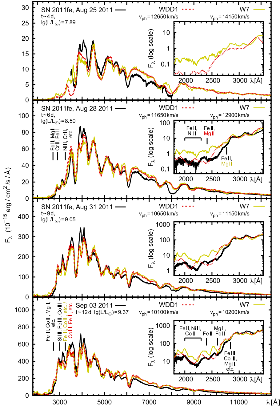
Figure 5. Spectra of SN 2011fe (black lines) compared to models based on the W7 and WDD1 density profiles (yellow/light grey, solid lines; red/grey, dotted lines, respectively). Insets show the UV in more detail (with logarithmic flux axis). The models have been reddened by E(B - V)_{\text{host}} = 0.014 mag. The ions responsible for the most prominent UV features in our model are marked, in order of importance.
