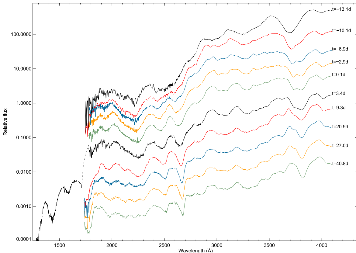
Figure 1. A time series spectral sequence of the UV portion of the HST spectra of SN 2011fe. Spectra have been corrected for MW extinction, corrected to the rest frame, and had UV ISM absorption lines removed. The phase of each spectrum, marked in days relative to maximum light in the rest-frame B band, is reported on the right. Each spectrum has been offset arbitrarily for presentation purposes.
