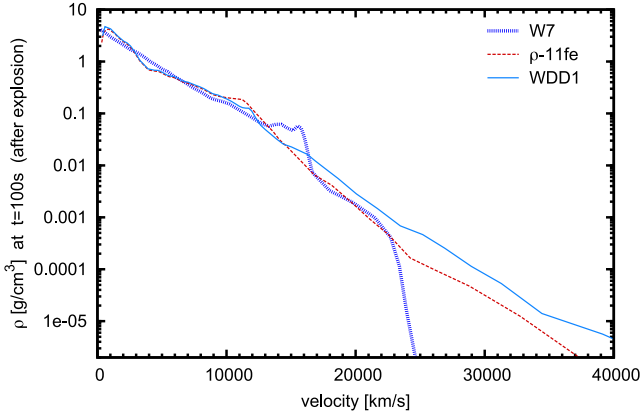
Figure 3. The SN ejecta density profiles of the W7 and WS15DD1 (WDD1) models discussed in Section 4.4 (Iwamoto et al. 1999), and of the \rho -11fe model constructed to optimize the comparison between the synthetic spectra and observed data (Section 5.3).
