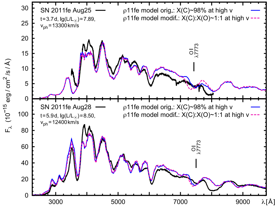
Figure 12. Effect of oxygen in the outermost layers of the model: the earliest two spectra of SN 2011fe (black) compared to \rho -11fe models. A spectrum where the outer layer is almost exclusively composed of carbon ( \sim 98 per cent by mass, blue/grey, solid lines) fits the observed O I \lambda 7773 line reasonably well, much better than a model where C and O have the same abundances at v > 19\,400 km s ^{-1} (red/grey, dotted lines). In the later spectrum the difference is already much smaller.
