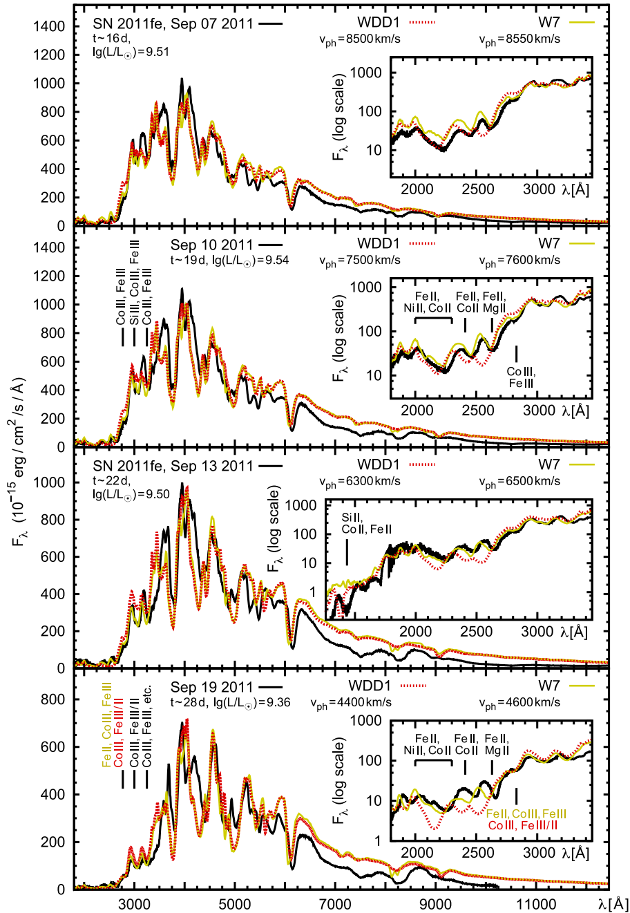
Figure 6. The W7 and WDD1 model sequences, continued Fig. 5.
