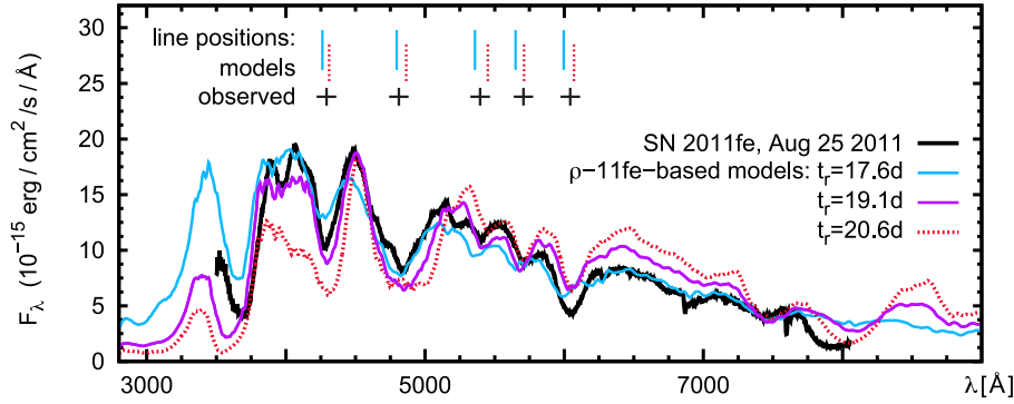
Figure 7. Early-time models for SN 2011fe based on the \rho -11fe density profile, assuming different rise-times t_r between 17.6 d and 20.6 d. The optimum rise-time is determined by comparing the positions of prominent features in the optical between observed spectrum (black crosses) and models (light blue/grey, solid lines for 17.6 d; purple/dark grey, solid lines for 19.1 d; red/dark grey, dotted lines for 20.6 d) – analogous to Fig. 4.
