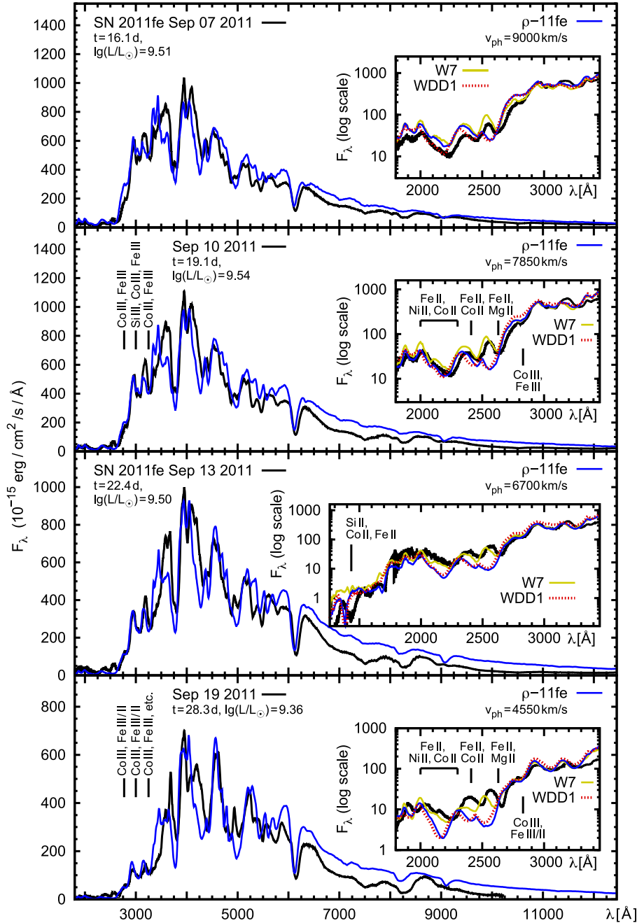
Figure 9. The \rho -11fe model sequence, continued from Fig. 8.
