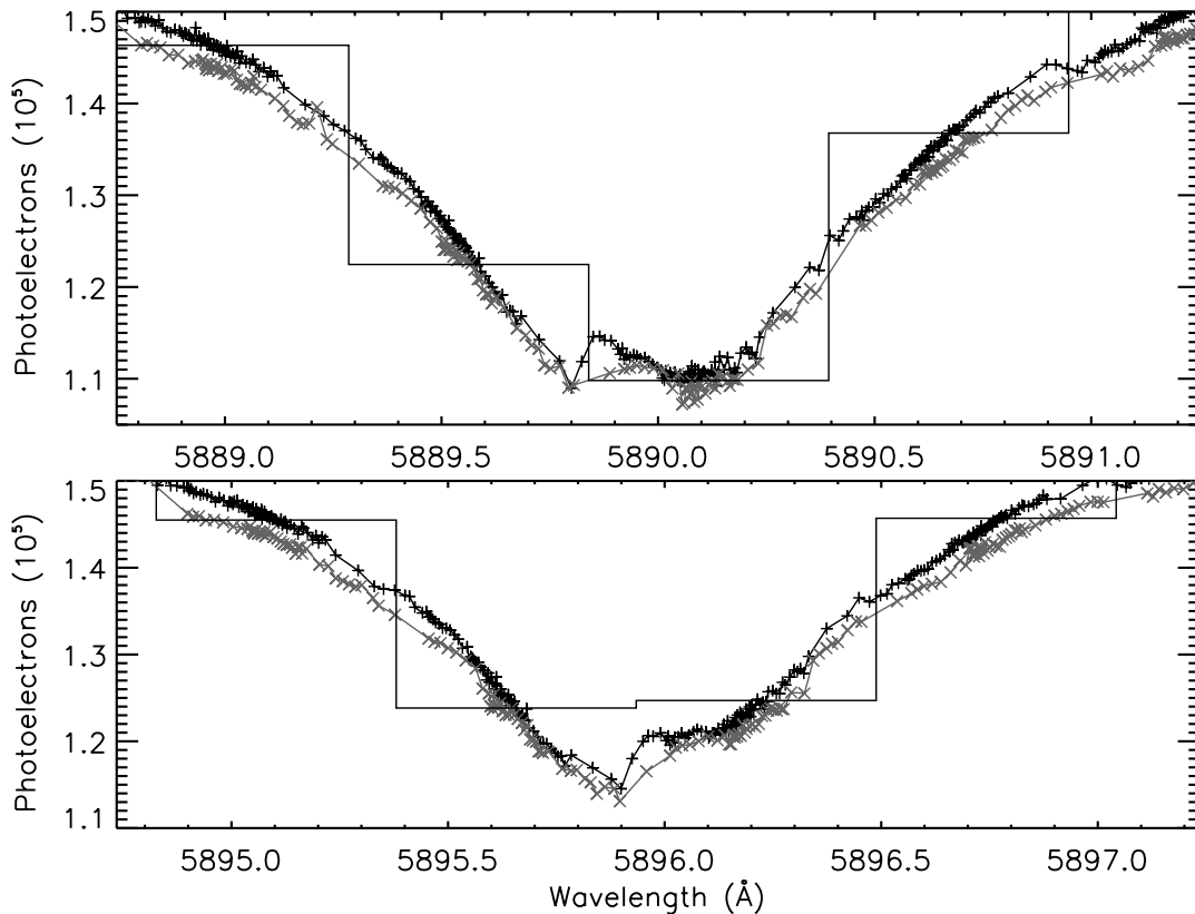
FIG. 1.—G750M spectra of the Na D2 (top) and D1 (bottom) line cores. Plotted are all of the out-of-transit spectra (black plus signs), as well as the in-transit spectra (gray crosses). The uncertainty in counts for each point is dominated by photon noise (approximately \pm 400 photoelectrons) and is smaller than the plotted symbol size. The first out-of-transit spectrum in the series is plotted in histogram mode to show the size of each pixel, 0.554 \text{ \AA} . Plotted together, each individual spectrum's Doppler and pixel shifts (accurate to \sim 0.1 pixel) effectively add up to better sample the PSF of the stellar absorption line profile. The \sim 1.5\% difference in flux during transit can be seen in the flux difference between the two spectra. However, the region showing contamination from 5889.5 to 5889.7 \text{ \AA} and from 5895.5 to 5895.8 \text{ \AA} shows little to no difference in flux during transit. This region shows variations with the HST orbital period, which we attribute to terrestrial-based sodium contamination.
