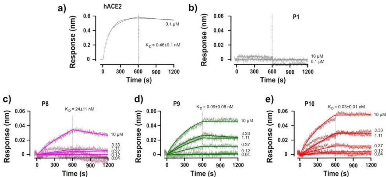
Fig. 4 Helical peptide-mimics of hACE2 strongly bind to the spike RBD. The Fc-tagged 2019-nCoV RBD-SD1 (Sanyou Biopharmaceuticals Co. Ltd) was immobilized to an anti-human capture (AHC) sensorchip (FortéBio) using an Octet RED96e system (FortéBio). The sensorchip was then dipped into a 0.1 \mu\text{M} solution of hACE2 (Sanyou Biopharmaceuticals Co. Ltd, His Tag), b 0.1 or 10 \mu\text{M} solution of P1 , or a range of concentrations (1 in 3 dilutions starting from 10 \mu\text{M} , i.e., 41 nM, 123 nM, 370 nM, 1.1 \mu\text{M} , 3.3 \mu\text{M} , and 10 \mu\text{M} ) for c P8 , d P9 , and e P10 to measure association rates before being dipped into a well containing only running buffer to measure dissociation rates. Data were reference subtracted and fitted to a 1:1 binding model using Octet Data Analysis Software v10.0 (FortéBio). All figures are representative of at least two independent experiments. K_D values were calculated from Supplementary Table 6.
