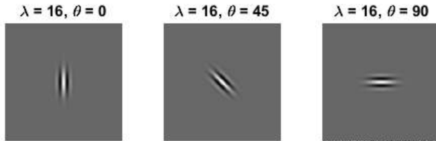
Figure 3.6: Change of real part of Gabor Kernel with Orientation.
