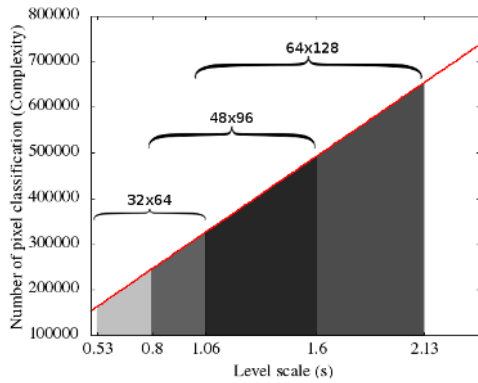
Fig. 5. In red : the growth of the complexity. From scale 0.53 to 1.06 : the complexity of a 32 \times 64 window scan, for instance.
