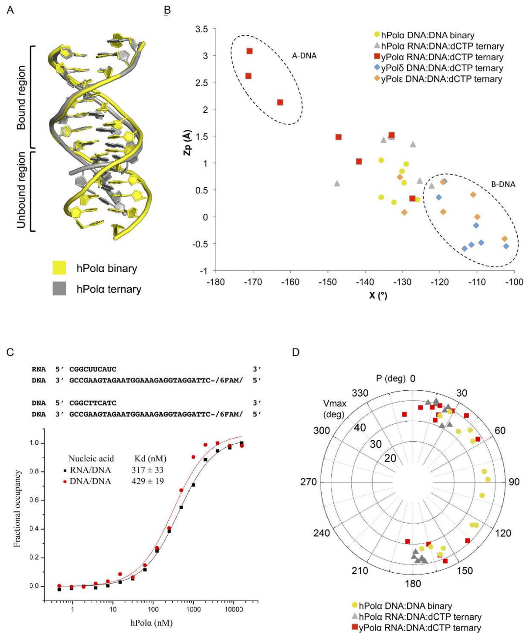
Figure 4. Conformation of nucleic acid. (A) Comparison of the DNA conformations of the hPolα binary complex (yellow) and the hPolα ternary complex (gray). The bound and unbound regions are marked in the figure. (B) Scatter plot of Z_p , the mean z-coordinate of the backbone phosphorous atoms with respect to individual dinucleotide reference frames, against the mean value for the four \chi torsion angles at each dinucleotide step. The values for 7 DNA:DNA base steps bound to hPolα in the binary complex are shown as yellow circles. The 7 RNA:DNA base steps bound to hPolα in the ternary complex (PDB code 4 QCL) are shown as gray triangles. The values for RNA:DNA base steps bound to yPolα (red squares), DNA:DNA steps bound to yPolδ (blue diamonds) and DNA:DNA steps bound to yPolε (orange diamonds) are also plotted. (C) Binding affinities of hPolα for DNA/DNA and RNA/DNA measured by a fluorescence anisotropy assay. The fraction of DNA/DNA or RNA/DNA bound is plotted versus hPolα concentration (logarithmic scale) in order to determine the dissociation constants. (D) Distribution of the pseudorotational phase angle P and puckering amplitude v_{max} of the base steps in contact with hPolα in the binary complex (yellow circles), with hPolα in the ternary complex (gray triangles) and with yPolα in the ternary complex (red squares).
