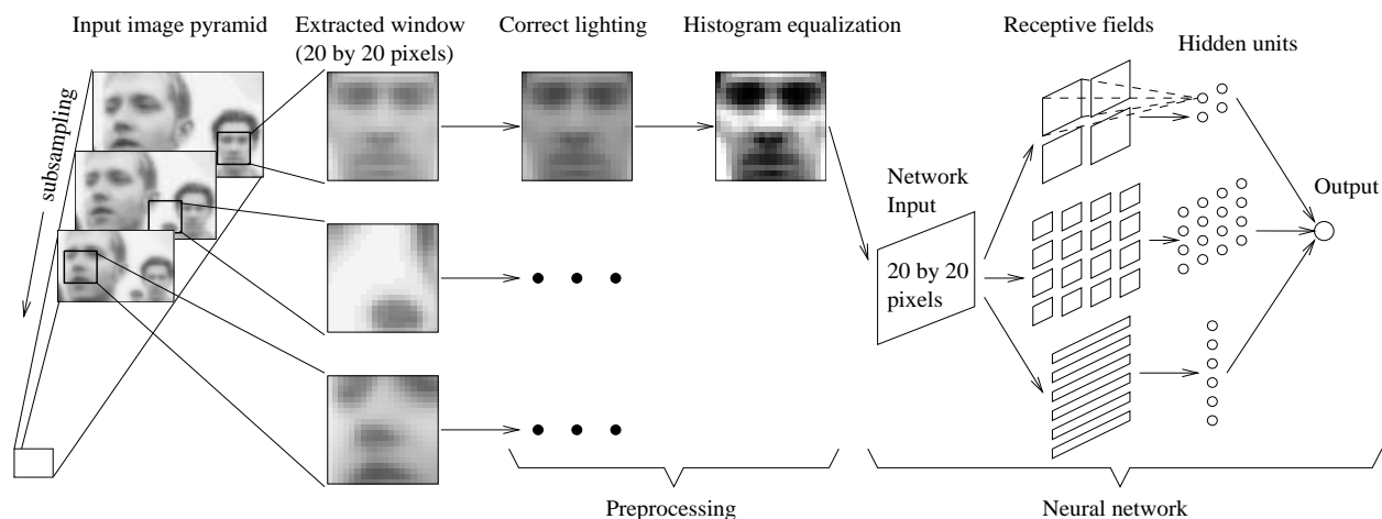
Figure 1: The basic algorithm used for face detection.
