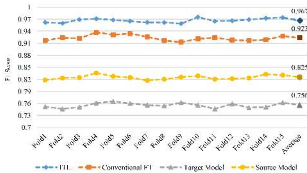
Fig. 11. Results of the leave two-individual-out cross-validation when there are 100 samples per class per person.
