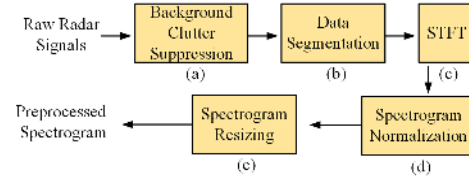
Fig. 2. Pipeline of radar raw signal preprocessing. (a) MTI is used on the raw radar signals for background clutter suppression. (b) Processed radar data is divided into several segments of 1 s with an overlap of 0.36 s between adjacent segments. (c) STFT is applied to transform the radar signals into 2-D complex data. (d) 2-D complex data are normalized, and the modules are obtained to form a spectrogram. (e) After resizing, the preprocessed spectrograms are obtained and used for further experiments.
