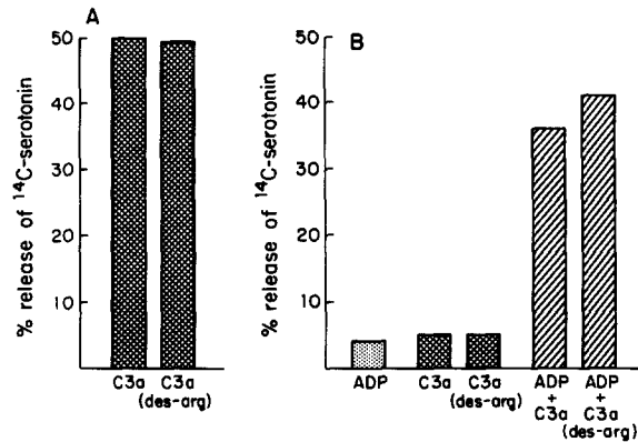
FIGURE 4. (A) Release of platelet serotonin mediated by C3a and C3a des-arg at 10^{-11} M. (B) Release of platelet serotonin mediated by ADP ( 10 \mu\text{M} ); C3a or C3a des arg ( 2 \times 10^{-12} M) singly; or ADP together with C3a or C3a des arg at the same concentrations.
