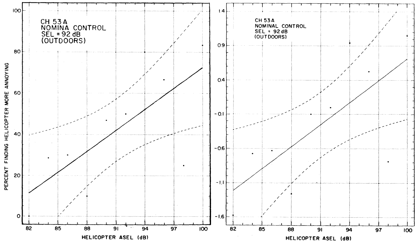
b. Same data converted to Z-scores.
