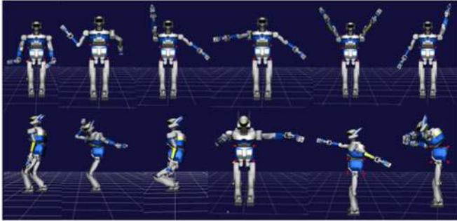
Fig. 2. Examples of exciting trajectories executed by the HRP-2 humanoid robot.
