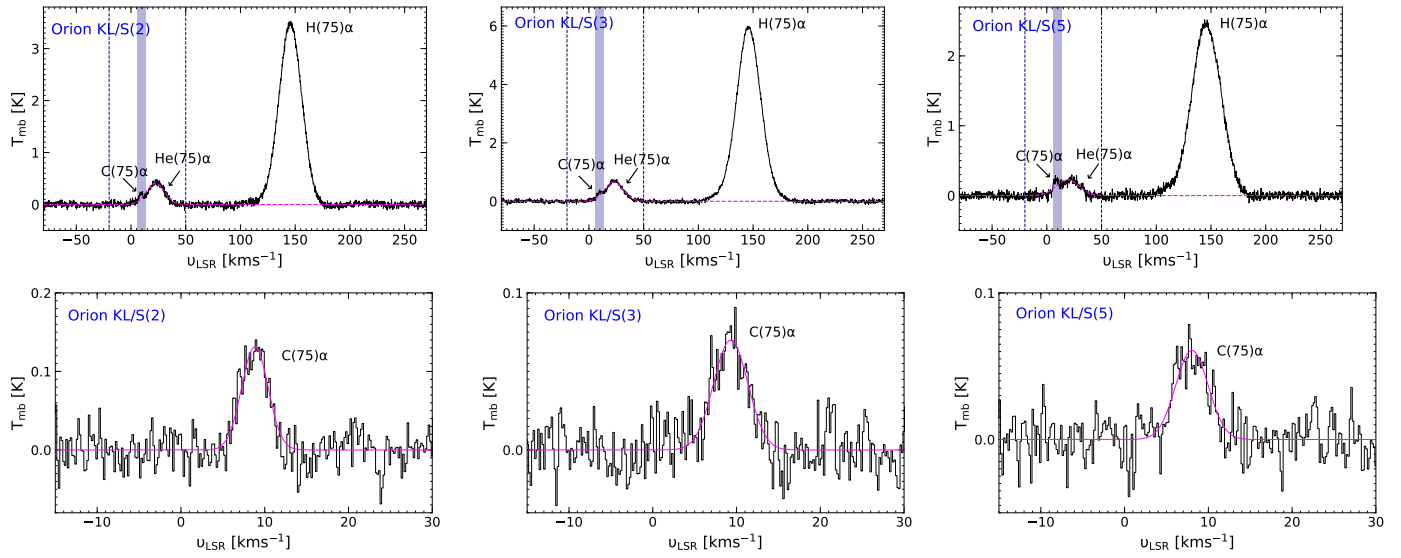
Fig. C.1. Top: H-, He-, and CRRLs toward different Orion KL/S OSO pointing positions, with the Gaussian fit to the He-RRRL displayed by the dashed magenta curve. Bottom: resulting CRRL with the Gaussian fit to the profile displayed in magenta. The velocity scale is given with respect to the CRRL.
