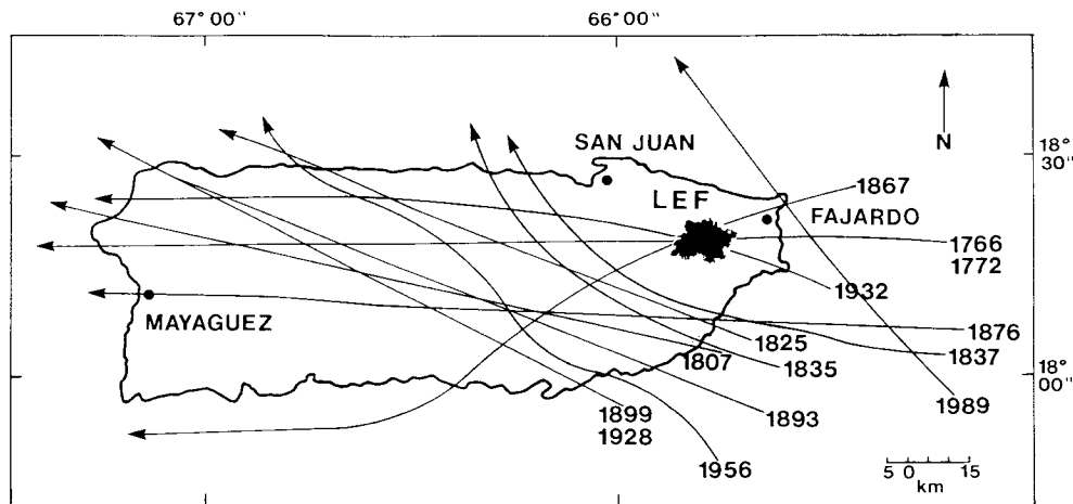
FIG. 1. Puerto Rico. Tracks of severe hurricanes since 1700 (adapted from Salivia 1950, Weaver 1987). LEF = Luquillo Experimental Forest. 1989 = Hurricane Hugo.
