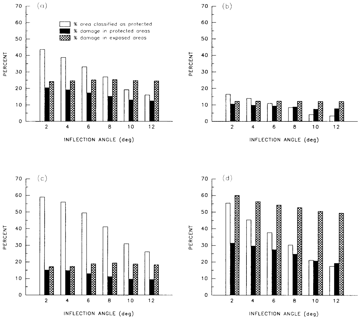
FIG. 12. Forest damage from Hurricane Hugo and predicted exposure for different sections of the Northern LEF study area and different inflection angles. Wind direction = 340°. (a) Entire study area. (b) West section. (c) Central section. (d) East section.
