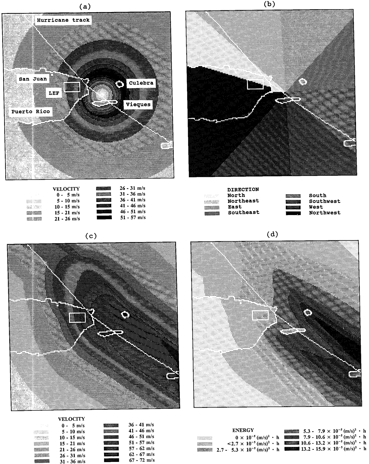
FIG. 9. Predicted wind over a 180 × 180 km grid on 18 September 1989 during Hurricane Hugo. Cell size = 1 × 1 km. (a) Predicted sustained wind velocity and (b) predicted sustained wind direction at 1200 UTC (for “UTC” see Table 3). (c) Predicted maximum wind gust velocity and (d) predicted total energy of sustained winds of gale strength (17 m/s) or greater over a 24-h period (time step = 2 min).
