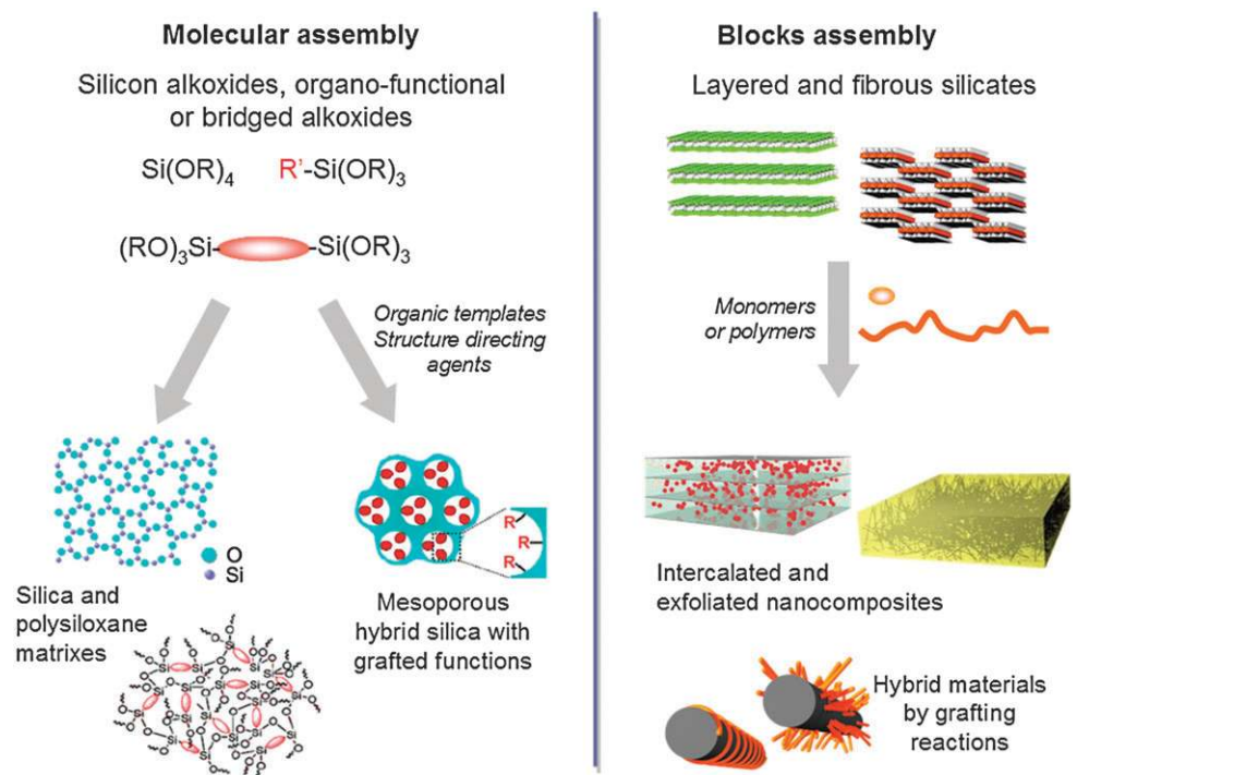
Fig. 2 Schematic representation of bottom-up strategies involving molecular-assembly or blocks-assembly.
