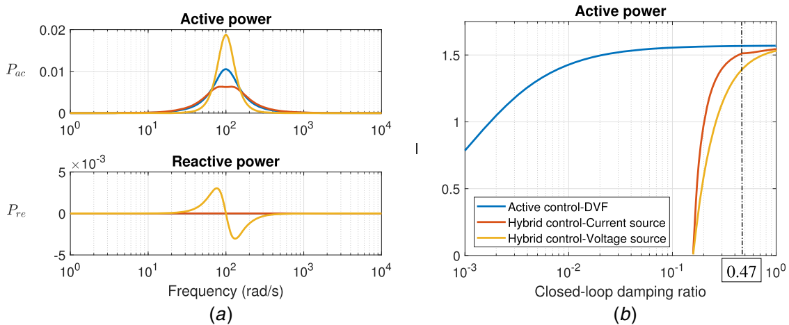
Fig. 11 Comparison between the purely active control system (DVF) and the hybrid control systems: (a) active and reactive power for a specific closed-loop damping ratio ( \approx 47\% ) and (b) the normalized mean square value of the active power I versus the closed-loop damping ratio (dash-dotted line shows the 0.47 damping ratio)
