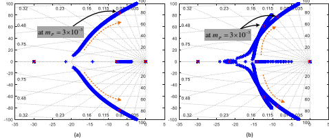
Fig. 4 Dominant system eigenvalues when 0.5 \times 10^{-4} > m_p > 5 \times 10^{-3} and lines inductances are (a) neglected (b) L_{Line1} = 1mH and L_{Line2} = 2mH
