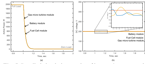
Fig. 5 Detailed simulation results of inverter's power and DC link voltage responses under load change when identical distribution lines are used
