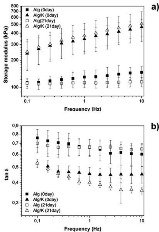
Fig. 8 DMTA scans of Alg and Alg/K hydrogels immediately after preparation and after 21 days of incubation in DMEM: (a) storage modulus (kPa); (b) \tan \delta .
