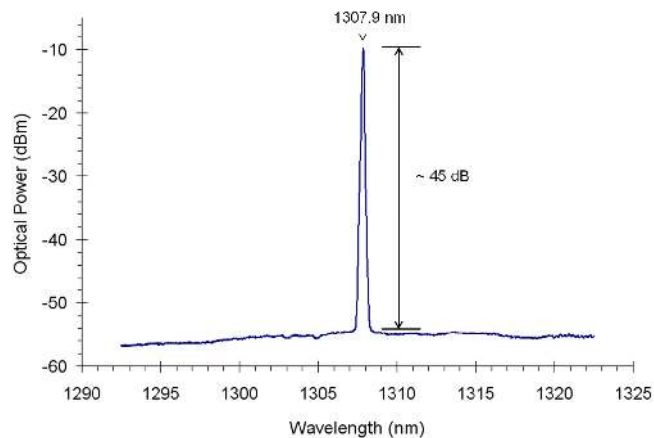
Fig. 6. Optical spectra of the hybrid DFB laser (CW regime, 100 mA injected current).
