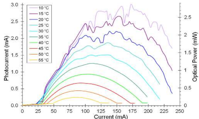
Fig. 5. Detected photocurrent vs. drive current ( I_{\text{ph}}-I ) plots of the hybrid DFB laser in CW regime (in a temperature range from 10 ^{\circ}\text{C} to 55 ^{\circ}\text{C} ). The right axis shows the optical power, estimated using 1.05 A/W responsivity for the integrated photodetector.
