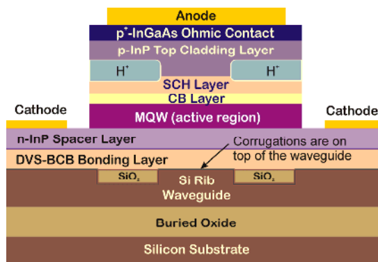
Fig. 1 Cross-section of an evanescent, hybrid III-V/Si DFB laser based on DVS-BCB bonding (SCH: separate confinement heterostructure; CB: carrier blocking; MQW: multi-quantum well). Corrugations are fabricated on top of the Si rib waveguide.
