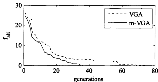
Figure 3.41 Fitness value change against generations
