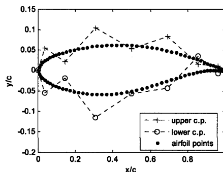
Figure 3.1 An airfoil in Bezier form.
