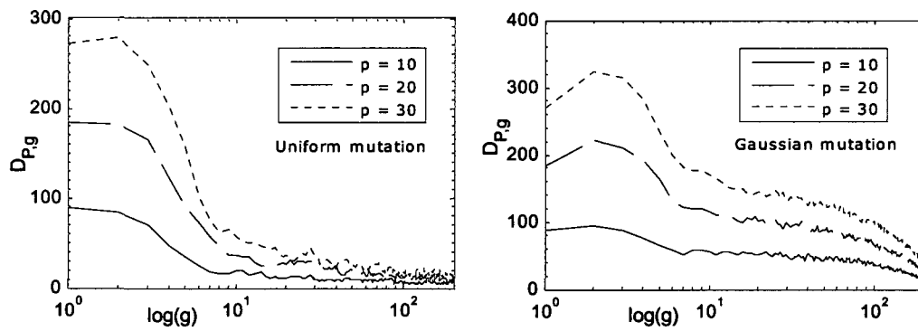
Figure 2.7 The diversity and population size relationship in accordance with Eq. (2.34).
