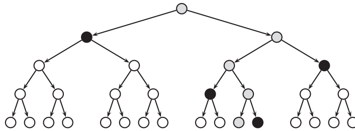
Fig. 2. Search tree example. Assume that the solution highlighted by light gray nodes is the unique optimal solution. Moreover, black nodes indicate that bounding information excludes them from the search process.
