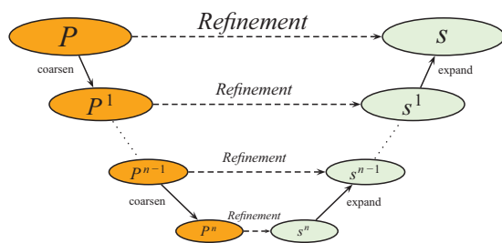
Fig. 1. The principle of a multilevel technique. The original problem instance is labelled P . This problem instance is iteratively simplified until a stopping criterion is satisfied at some level n corresponding to instance P^n . Then, a metaheuristic may be applied for the generation of a solution s^n to instance P^n , which is subsequently expanded into a solution s^{n-1} to instance P^{n-1} of level n-1 . The refinement of solution s^{n-1} may be done by a metaheuristic again. This process is stopped once a solution to the original problem instance has been obtained.
