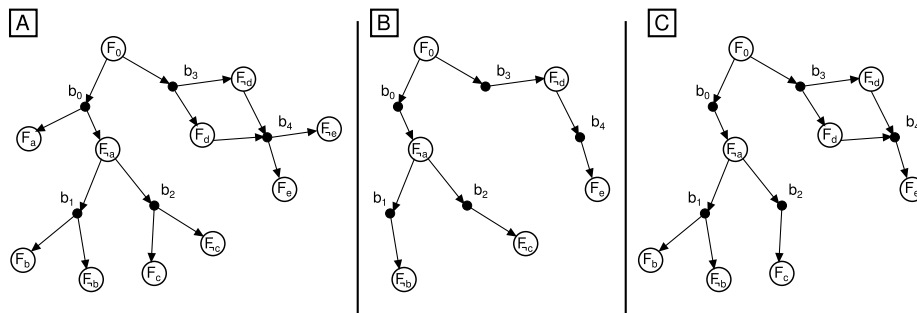
Figure 4.10: (A) BFG for the graph in Figure 4.6 - (B) the s -tree associated to the scenario \neg a \neg b \neg c \neg d e - (C) a subgraph (set of s -trees) associated to scenarios where \neg ace holds
