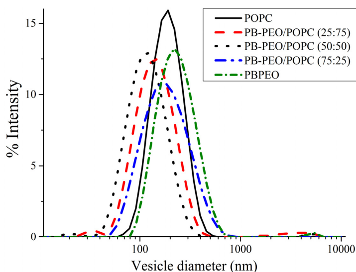
Figure 4. Intensity-weighted hydrodynamic diameter of extruded vesicles prepared from POPC, PB-PEO/POPC (75:25), PB-PEO/POPC (50:50), PB-PEO/POPC (25:75), and PB-PEO, as measured by DLS. All vesicles show a single unimodal population.
