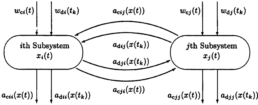
FIGURE 1 Nonlinear hybrid compartmental interconnected subsystem model.
