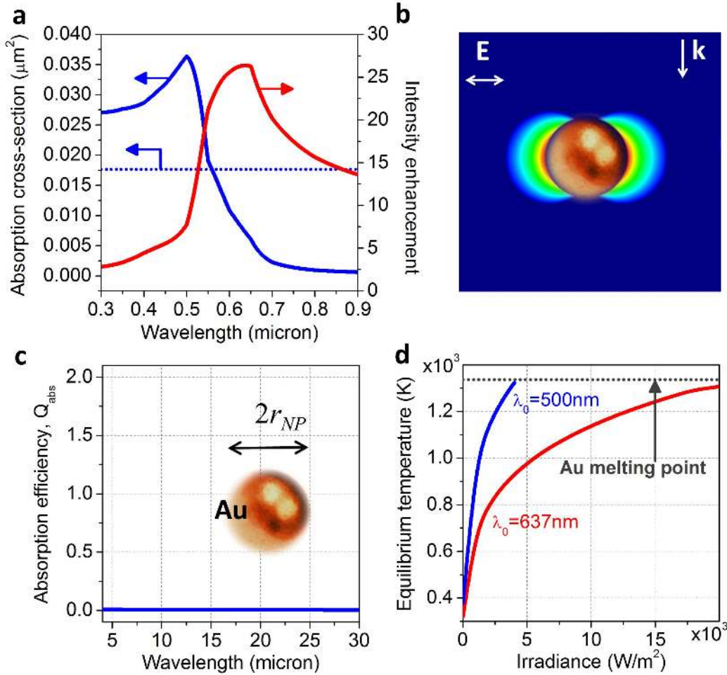
Figure 1. Noble metal plasmonic nanoantennas amplify light intensity yet heat up by absorbing photons. (a) Local intensity enhancement, |E|^2/|E_0|^2 (red line) and absorption cross-section (blue line) of an isolated 150nm-diameter Au nanoparticle in vacuum. The nanoparticle geometrical cross-section is shown for comparison (dotted blue line). (b) Electric field intensity distribution in the near field of Au nanoparticle at the wavelength of the field intensity peak in Fig. 1a (637nm). Here and in Fig. 2a the local electric field intensity is calculated inside the nanoparticle plasmonic hot-spot shown in Fig. 1b 0.5nm away from the Au surface. (c) Infrared frequency spectrum of the absorption (i.e., also emission) efficiency of the Au particle. The inset shows the particle schematic. (d) Equilibrium temperature of the particle reached under steady-state illumination by a monochromatic plane wave with varying photon flux and with a frequency centered either at the particle absorption peak of 500 nm (blue line) or at the particle intensity peak of 637nm (red line). The melting point of Au (1337K) is shown as a gray dashed line for reference.
