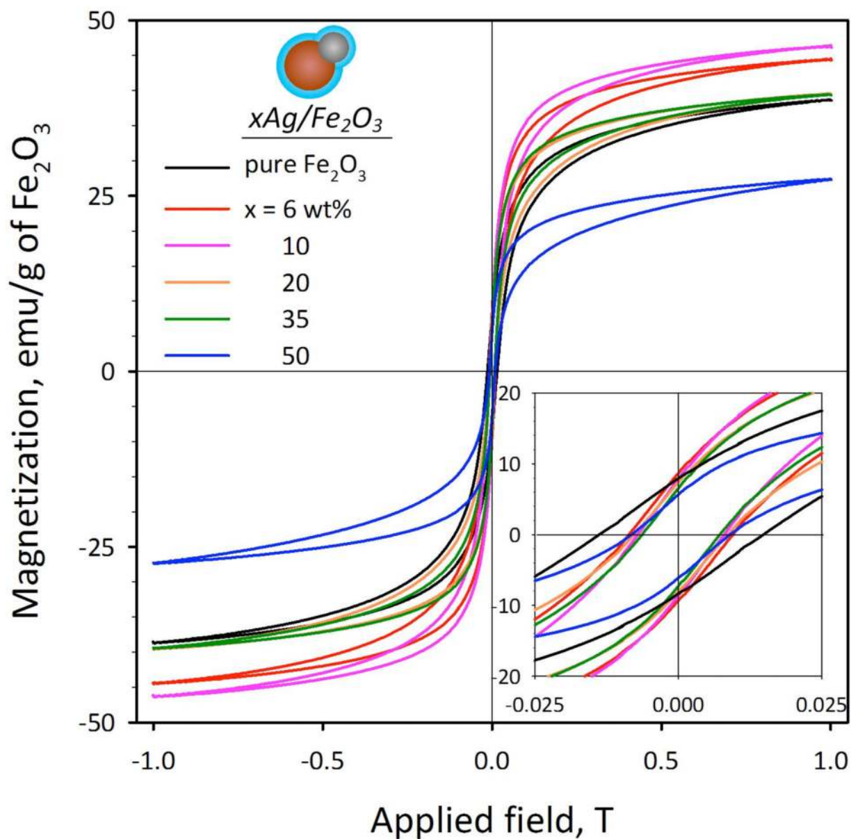
FIGURE 2. Magnetization curves of the \text{SiO}_2 -coated x\text{Ag}/\text{Fe}_2\text{O}_3 samples. The magnetization values have been normalized for an equal mass of \text{Fe}_2\text{O}_3 . The inset shows a magnification at low magnetic fields highlighting the coercivity and remanence of the particles. The hybrid \text{SiO}_2 -coated \text{Ag}/\text{Fe}_2\text{O}_3 nanoparticles exhibit a near superparamagnetic behavior.
