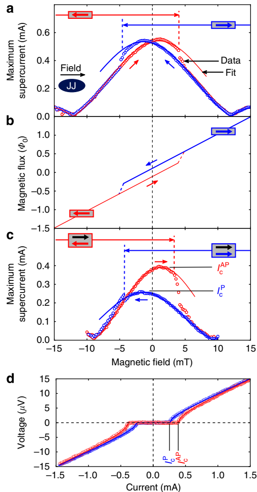
Figure 2 | Electrical measurement results of S-PSV-S JJs with magnetic field. (a) Maximum supercurrent versus magnetic field of a JJ with zero Ni thickness ( d Ni ≈ 0) in the PSV barrier structure, Ni 0.7 Fe 0.17 Nb 0.13 (2.1 nm)/Cu(5 nm)/Ni( d Ni ). The JJ design is a 0.9 μm × 1.8 μm ellipse and the magnetic field is applied along the long axis of the ellipse (inset). (b) Total magnetic flux in the junction versus field inferred from the offsets in the Fraunhofer-like patterns in a. (c) Maximum supercurrent I m versus magnetic field of the S-PSV-S device with d Ni = 1 nm. The JJ design is a 1.2 μm × 2.4 μm ellipse. (d) Current versus voltage of the device used in c measured at the magnetic field giving the peak I m for each state. The measurement temperature is 4 K. I c P and I c AP are the critical currents with the P and AP magnetization states of the PSV barrier, respectively. Symbols are measured data and lines are fits. The magnetization states are labelled by coloured and black arrows in the illustrated boxes above the plots for the Ni 0.7 Fe 0.17 Nb 0.13 and the Ni layers, respectively.
