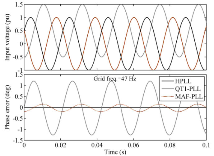
Fig. 12. Steady-state simulation results when a large dc offset exists in the PLL input.
