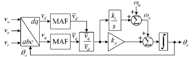
Fig. 1. Structure of the standard MAF-PLL.
