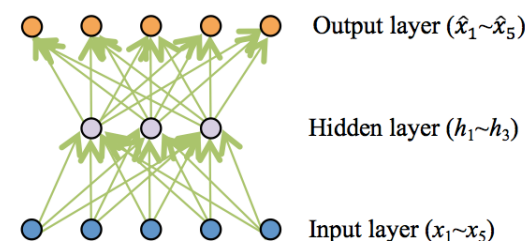
FIGURE 2. Autoencoder operation.
