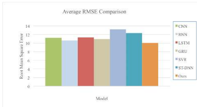
FIGURE 7. Average RMSE comparison.
