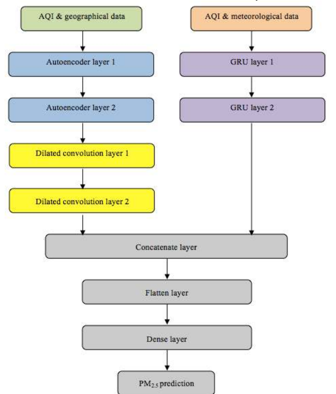
FIGURE 1. Framework diagram.
