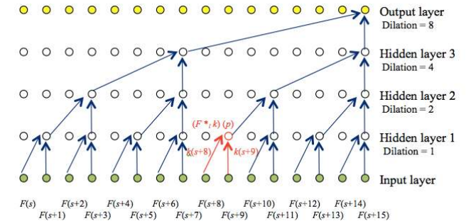
FIGURE 4. Dilated convolution operation.
