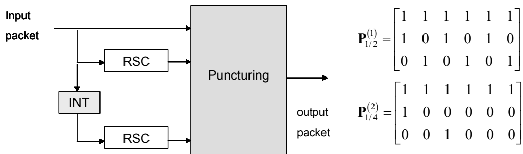
Figure 5 - Punctured turbo code encoder
