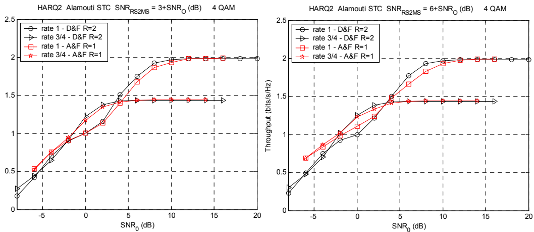
Figure 13 - Throughput for C-D&F and C-A&F schemes with HARQ-II with RCPTC of rates \{3/4, 1\} using Alamouti STC (ZF), for SNR_{RS2MS}=3+SNR_0 (left) and SNR_{RS2MS}=6+SNR_0 (right). SNR_{BS2RS}=SNR_{BS2MS}=SNR_0 .
