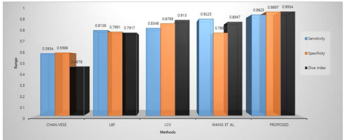
Fig 11. Comparative analysis of BRATS 2015 challenge dataset in terms of sensitivity, specificity and Dice index metrics.
