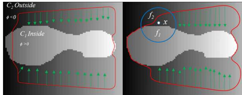
Fig 2. Graphical representation of taking intensity information, where c_1, c_2 are global and f_1, f_2 are local intensity means, green arrows represent the effect of geodesic term. a: First stage segmentation. b: second stage segmentation.
