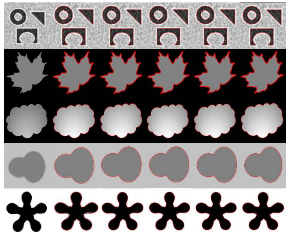
Fig 7. Segmentation results using the same accuracy level. Column(1): Original images. Column(2): Chan-Vese result. Column(3): LBF result. Column(4): LCV result. Column(5): Wang et al. result. Column(6): Proposed method result.
