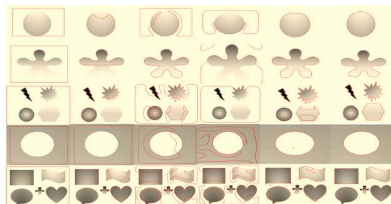
Fig 4. Segmentation results using images from different intensity variations. (a): original images with initial contours. (b): Chan-Vese result. (c): LBF result. (d): LCV result. (e): Wang et al. result. (f): proposed method result.
