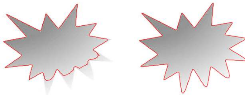
Fig 1. Intensity inhomogeneous image segmentation using. a: Chan-Vese method segmentation. b: LBF method segmentation.
