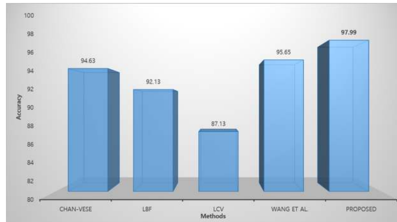
Fig 9. Segmentation accuracy of each method.
