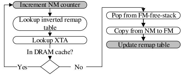
Figure 8: Allocating a sector in NM.
